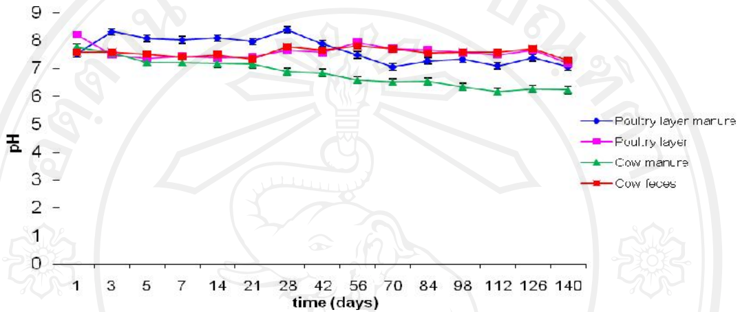
Figure 7 Changing of pH in composted and non-composted materials, the error bars represent the standard error.
