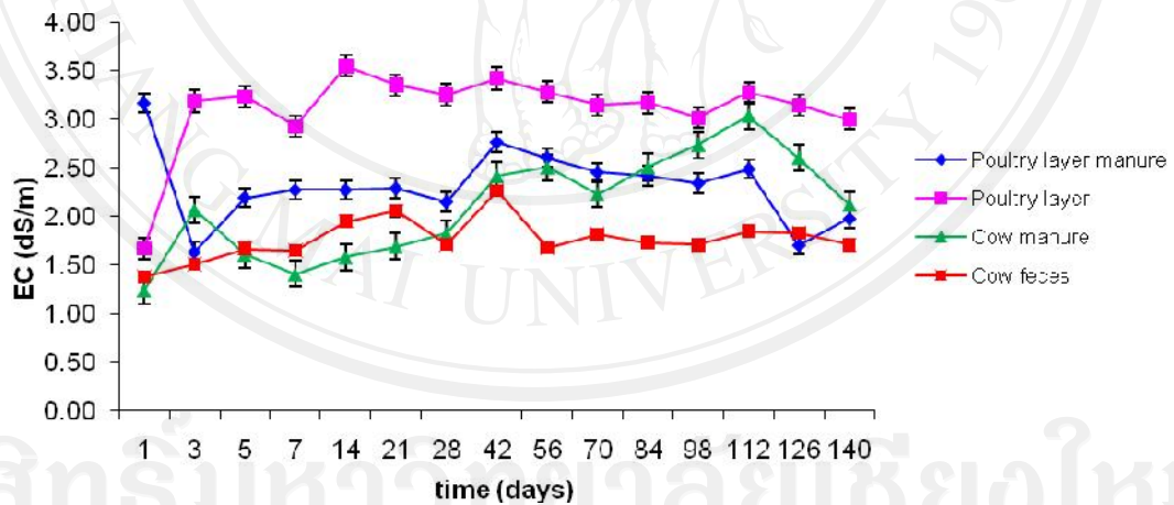
Figure 4 Changing of EC of composted and non-composted materials, the error bars represent the standard error.
