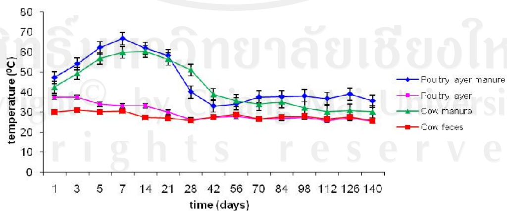
Figure 6 Changing of temperature in composted and non-composted materials, the error bars represent the standard error.
