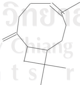
trans caryophyllene
