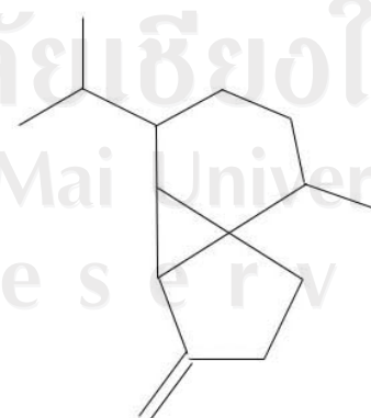
\beta -cubebene
