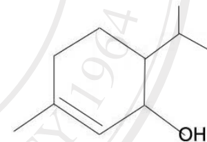
2-cyclohexen-1-ol, 3- methyl-6-(1-methylethyl)
