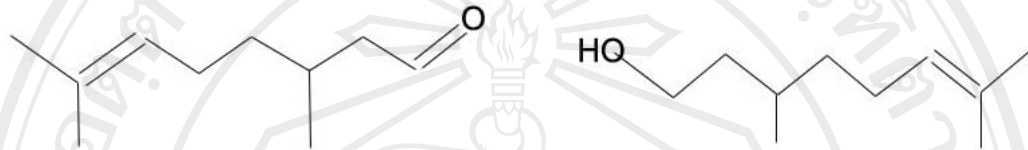
Citronellal
