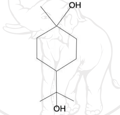
cyclohexanemethanol, 1-methyl-4-(1-methylethyl)
