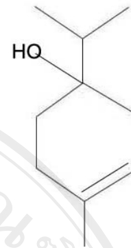
terpinene-4-ol
