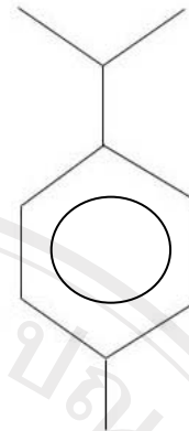
1-methyl-4-(1-methylethyl)-benzene
