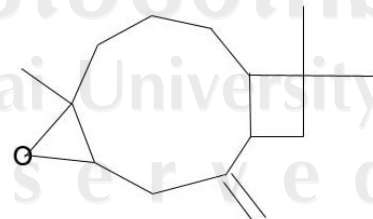
caryophyllene oxide
