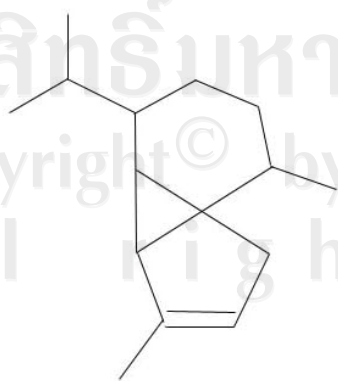
\alpha -cubebene
