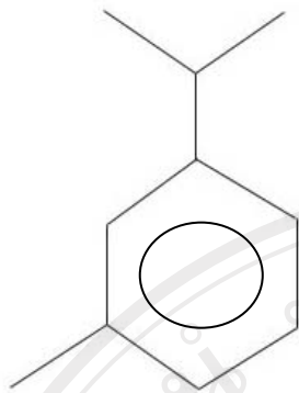
1-methyl-3-(1-methylethyl)-benzene
