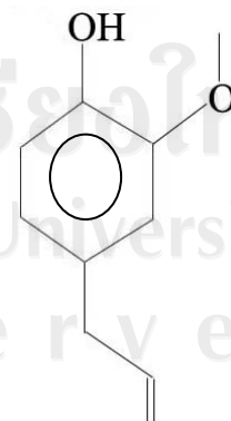
2-methoxy-4-(2-propenyl)
