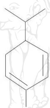
1-phellandrene
